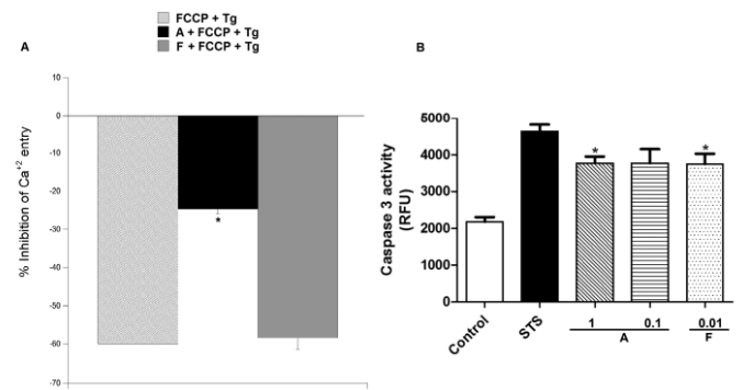
Figure 7. (A) Blockage of the FCCP inhibition of Ca 2+ entry after Tg-induced endoplasmic reticulum empty. Compound A inhibited the FCCP effect, whereas compound F did not affect the Ca 2+ entry decrease produced by FCCP. (B) Caspase-3 activity was measured as an apoptosis signal. Cotreatments of 0.5 μM STS and compounds A (1 and 0.1 μM) and F (0.01 μM) showed a decrease of the caspase-3 activity respect to cells only treated with STS. All values are shown in RFU and compared to cells treated with 0.5 μM STS. *p < 0.05. Data are mean ± SEM of three or more independent experiments.
