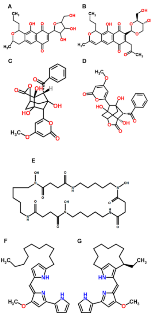
Figure 1. Compound structures.
